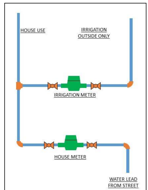
Irrigation Meter Diagram
